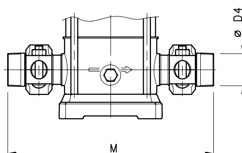
THREADED SLEEVES
