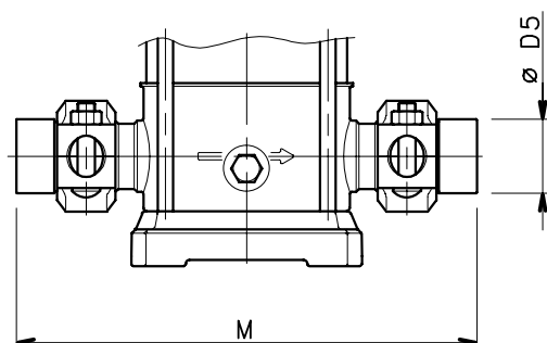
WELD-ON SLEEVES
