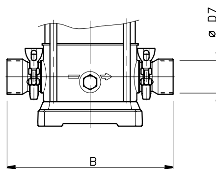
THREADED SLEEVES
