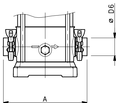
WELD-ON SLEEVES
